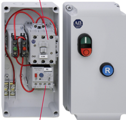
E1 Plus Electronic Overload Relay
